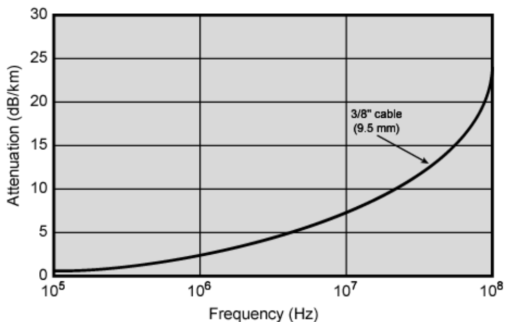
(b) Coaxial cable (based on [BELL90])
