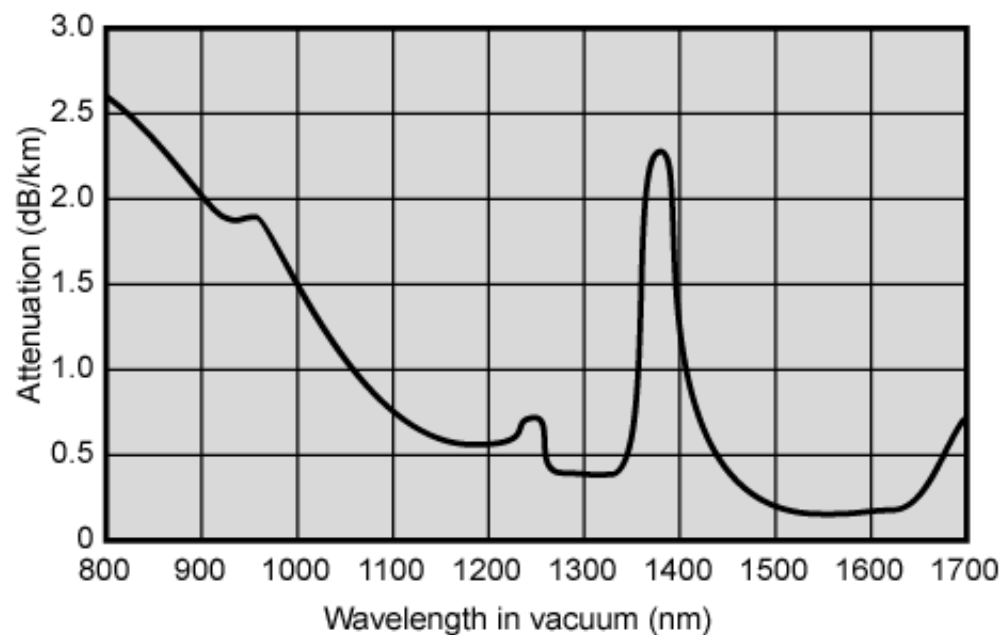
(c) Optical fiber (based on [FREE02])
